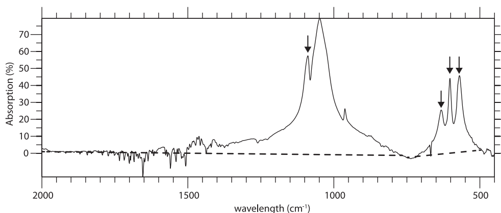
Fig. 3. IR absorption spectrum of AAR-8987. IR spectra of the bio-apatite bone fraction are represented by vibration bands of mainly \text{CO}_3 and \text{PO}_4 giving absorption peaks at 710, 874 and 1415\text{ cm}^{-1} and 565 , 603 and 1035\text{ cm}^{-1} of \text{CO}_3 and \text{PO}_4 respectively (Garvie-Lok et al., 2004). The crystallinity is a function of the extent of splitting of the two absorption bands at 603 and 565\text{ cm}^{-1} . Arrows shows the splitting in the IR spectrum indicating high crystallinity.
