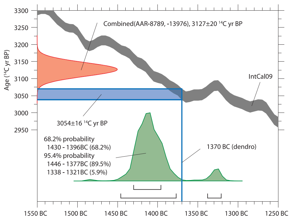
Fig. 2. IntCal09 radiocarbon calibration curve with \pm 1\sigma uncertainty lines (Reimer et al., 2009) and the calibrated age probability density function of the combined ^{14}\text{C} date of AAR-8789 and AAR-13976 determined by OxCal 4.10 (Ramsey, 2009). Using the radiocarbon calibration curve the dendrochronological coffin date 1370 BC is converted to the corresponding ^{14}\text{C} age of 3054 \pm 16 BP.
