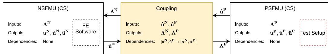
Fig. 13. Co-simulation scenarios that implements the setup described in Fig. 12. The dashed boxes represent the fact that NSFMU (respectively PSFMU) communicate with a FE Software (resp. the Test Setup), when the fmi2DoStep function is invoked.
