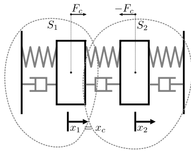
Fig. 8. Double mass-spring-damper.
