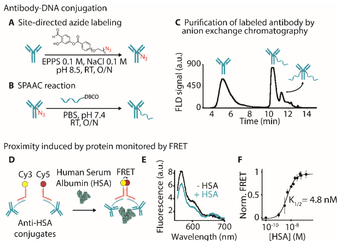
Figure 2. DNA-antibody conjugation and protein-induced proximity monitored by FRET. A) Site-directed labelling of a polyclonal antibody via reaction with a directing reagent bearing an azide handle. B) SPAAC reaction between the labelled antibody and a DBCO-modified DNA strand furnishes the DNA-antibody conjugate. C) Anion exchange chromatogram of the reaction mixture obtained from SPAAC reaction that allows the purification of the monolabelled conjugate. D) Design of a pair of fluorescently labelled DNA strands complementary to anti-HSA conjugates for the study of the proximity effect induced by HSA. E) Fluorescence spectrum of the system shown in (D) in the absence (black) and in the presence of HSA (blue). F) Titration of the system with increasing concentrations of HSA measured by FRET. The K_{1/2} is 4.8 nM. The fluorescence experiments were performed at 37 °C in 25 mM HEPES buffer pH 7.2, 0.1 M NaCl, 0.05% Tween20 at a fixed concentration of the fluorescently labelled strands (30 nM), anti-HSA conjugate (60 nM) in the absence and presence of HSA protein (60 nM, unless otherwise indicated). The experimental values reported in panel (F) represent averages of three independent measurements and the error bars reflect the standard deviations.
