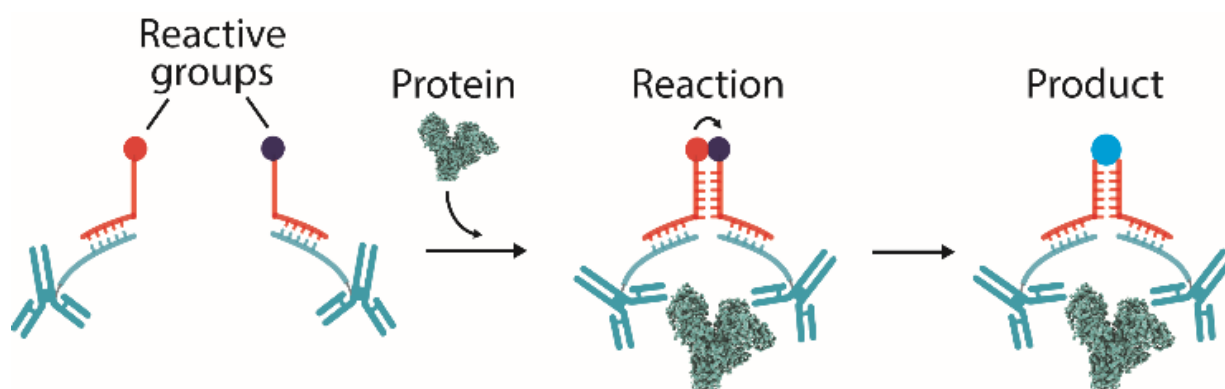
Figure 1. Strategy to achieve protein-templated reactions using DNA-antibody conjugates. Two complementary (10-bp) DNA strands (reactant strands, shown in red) are each conjugated at one end with a reactive group and at the other end they hybridize to a complementary (23-bp) DNA strand on an DNA-antibody conjugate (shown in blue). At low oligonucleotide concentrations (nM), duplex formation between the reactant strands is not favored and thus the reaction rate between the two reactive groups is negligible. Binding of the conjugates to different epitopes on the specific target protein dramatically increases the effective concentration of the reactant DNA strands. This protein-induced proximity effect enables the hybridization of the reactant strands followed by their reaction and subsequent formation of product. The scheme depicted is a simplified version (for the detailed design see Figure S1 in the Supporting Information).
