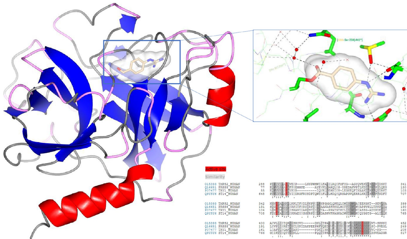
FIGURE 2 Camostat metabolite GBA binding to serine protease. Crystal structure of prostatic trypsin (3FVF) with camostat metabolite GBA covalently bound in the active site. Camostat mesylate and GBPA can be cleaved to form GBA. This cleavage process forms a covalently bound GBA to Serine in the active site. There is high similarity of the active site between the serine proteases, TMPS2 (TMPS2), Prostatic trypsin (PRSS8), Trypsin (TRY1) and Matriptase (ST14) that are all targets of camostat mesylate
