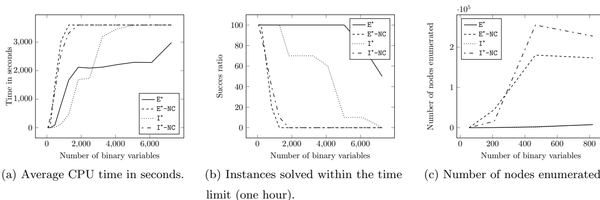
Figure 5 The effect of cutting planes.
