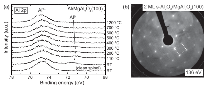
FIG. 3. (a) XPS spectra of the Al 2p region. (b) Normal incidence LEED pattern of s\text{-Al}_2\text{O}_3(100) .
