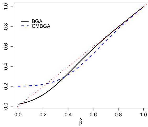
Figure 3: Shrinkage of slope parameter for \sigma_{\beta} = 0.2 and 5% level. Dotted line is 45° line.
