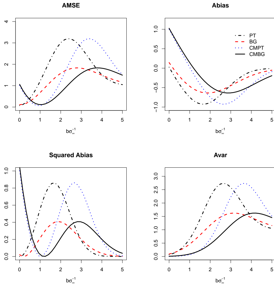
Figure 2: Comparison of asymptotic mean-squared error (AMSE), asymptotic bias (Abias), asymptotic square bias (Abias square), and asymptotic variance (Avar) as a function of b\sigma_\infty^{-1} for 1% significance level .
