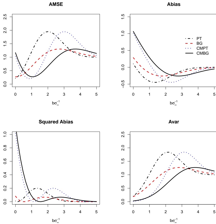
Figure 1: Comparison of asymptotic mean-squared error (AMSE), asymptotic bias (Abias), asymptotic square bias (Abias square), and asymptotic variance (Avar) as a function of b\sigma_{\infty}^{-1} for 5% significance level .
