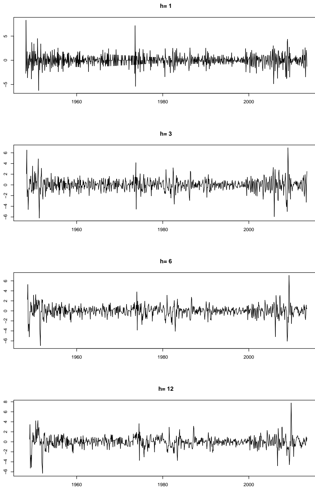
Figure 4: Time series of target variable \Delta\pi_t^h at the different forecasting horizons h .
