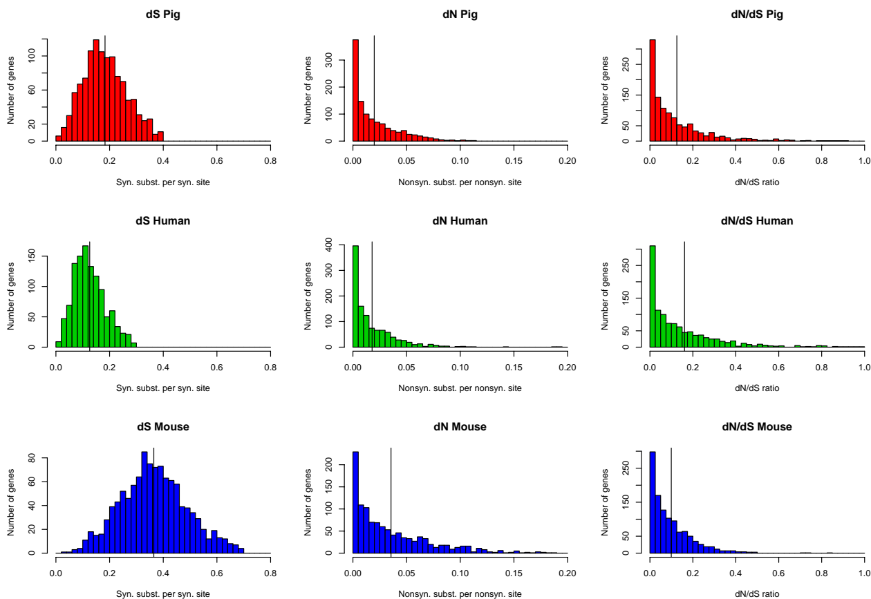
Figure 4 Evolutionary rates. Histograms of key parameters in the codon models. (a-c) The rate of synonymous substitutions per synonymous site (dS) in the pig, human and mouse lineage respectively. (d-f) The rate of nonsynonymous substitutions per nonsynonymous site (dN) in the pig, human and mouse lineage respectively. (g-h) The ratio of nonsynonymous substitutions to synonymous substitutions (dN/dS ratio) in the pig, human and mouse lineage respectively. The horizontal line represents the mean of the distributions.
