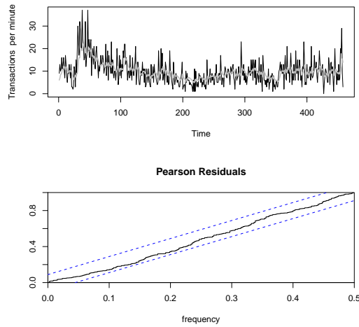
Figure 5: Top: Observed and predicted (grey) number of transactions per minute using (2). Bottom: Cumulative periodogram plot of the Pearson residuals.
