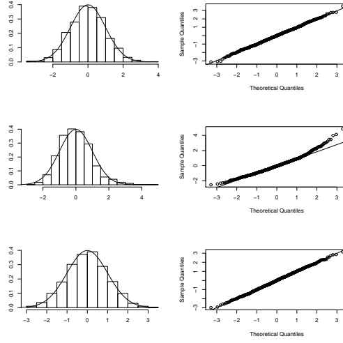
Figure 2: From top to bottom: Histograms and qq-plots of the sampling distribution of the standardized estimators of \hat{\theta} = (\hat{a}, \hat{c}, \hat{b}) for the exponential autoregressive model (5) when the true values are (d_0, a_0, b_0) = (0.25, 1, 0.65) and the parameter \gamma is assumed to be known and equal to 1. Superimposed is the standard normal density function. The results are based on 500 data points and 1000 simulations.
