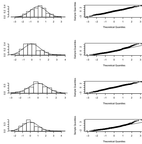
Figure 3: From top to bottom: Histograms and qq-plots of the sampling distribution of the standardized estimators of \hat{\theta} = (\hat{a}, \hat{c}, \hat{b}, \hat{\gamma}) for the exponential autoregressive model (5) when the true values are (d_0, a_0, b_0, \gamma_0) = (0.25, 1, 0.65, 1) . Superimposed is the standard normal density function. The results are based on 1500 data points and 500 simulations.
