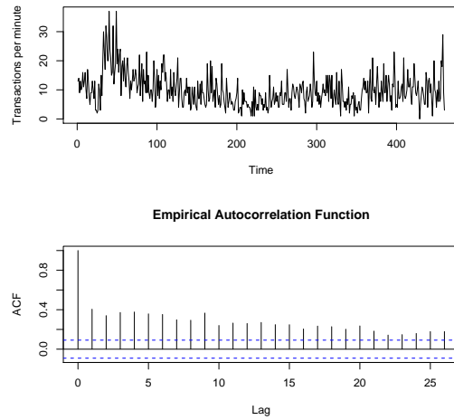
Figure 4: Number of transactions per minute for the stock Ericsson B during July 2nd, 2002. The bottom plot shows their autocorrelation function
