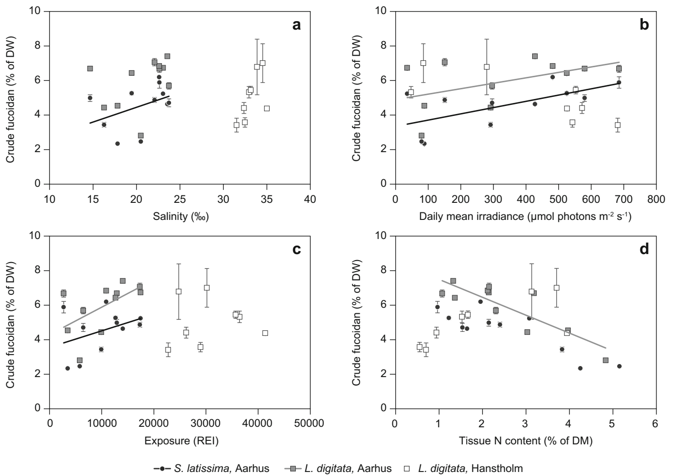
Fig. 4 The tissue content of crude fucoidan as a function of single environmental factors: a salinity; b irradiance; c exposure (relative exposure index (REI)); d tissue N content (% of DM). Data represent average \pm SE, n = 3 . Statistics are given in Table 4. Only significant relations are indicated by lines
