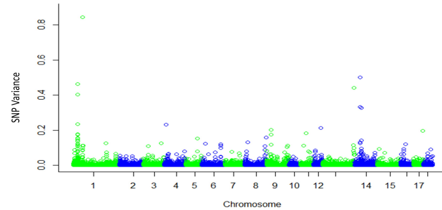
Figure 1: Manhattan plot of estimated SNP variance for RFI with BPL0.3
