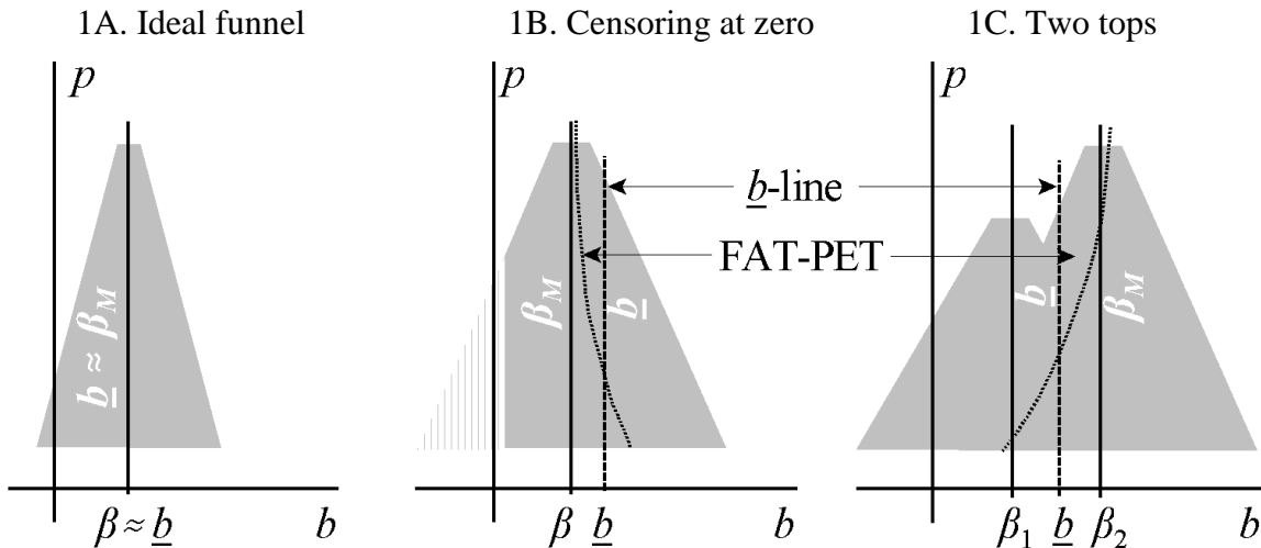
Figure 1. Funnels with typical forms affected by POCs
