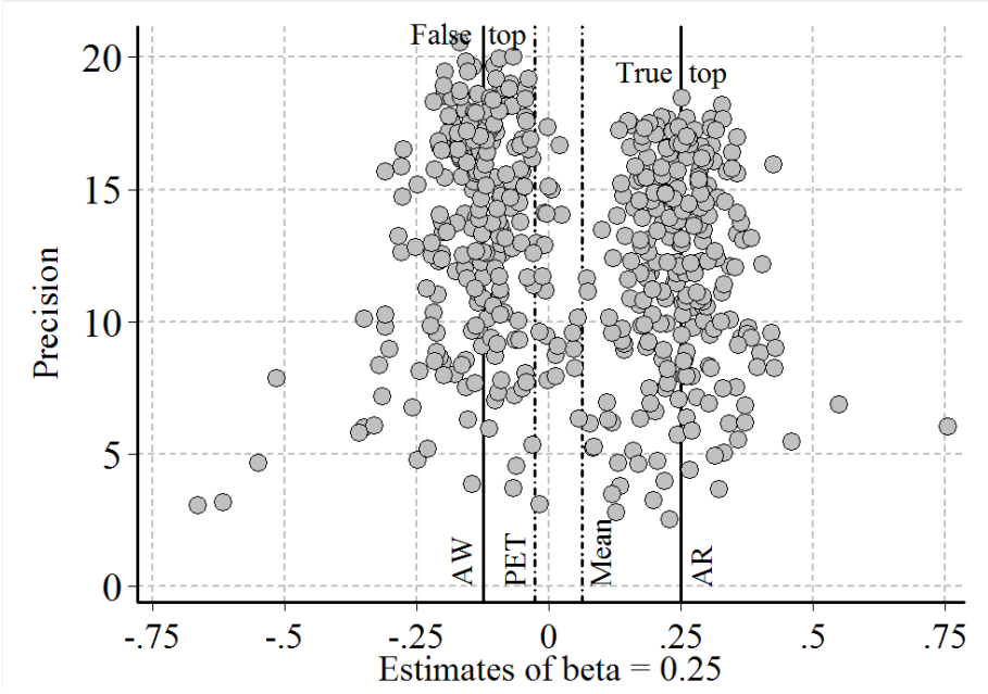
Figure 8. Case (3.3) without censoring
