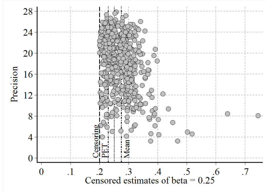
Figure 4. The funnel from Figure 3 censored at the censoring point C = 0.2
