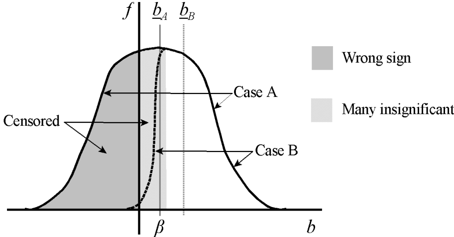
Figure 2. The frequency ( f ) of possible choices with the trove approach
