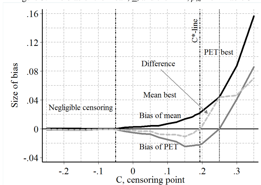
Figure 5. The bias of the mean, b , and the PET, \beta_M from Table 3
