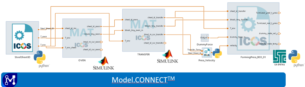
Figure 3: The connection diagram for the different components of the co-simulation
