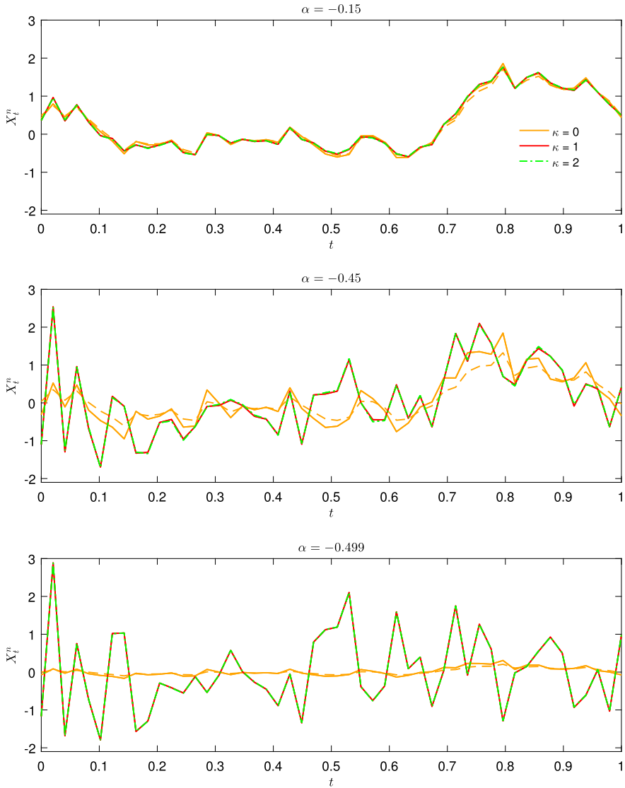
Fig. 2 Discretized trajectories of a BSS process, where g is the gamma kernel (Example 2.3), \lambda = 1 and \sigma_t = 1 for all t \in \mathbb{R} . Trajectories consisting of n = 50 observations on [0, 1] were generated with the hybrid scheme ( \kappa = 1, 2 and \mathbf{b} = \mathbf{b}^* ) and Riemann-sum scheme ( \kappa = 0 and \mathbf{b} = \mathbf{b}^* (solid lines), \mathbf{b} = \mathbf{b}_{\text{FWD}} (dashed lines)), using the same innovations for the driving Brownian motion in all cases and N_n = \lfloor 50^{1.5} \rfloor = 353 . The simulated processes were normalized to have unit (stationary) variance
